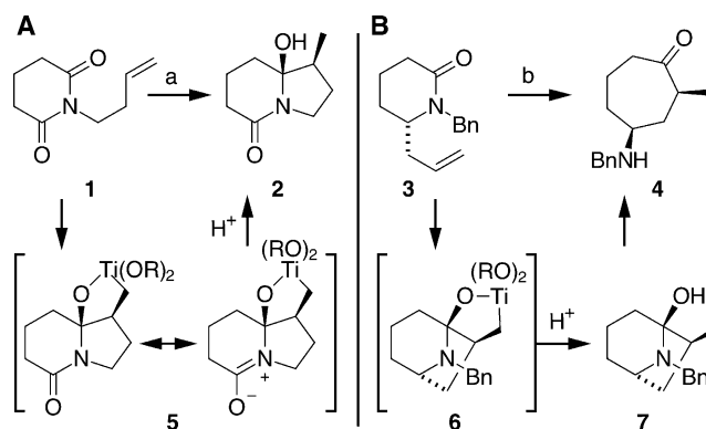
Scheme 2. Interrupted Kulinkovich–de Meijere reactions. A) Cha's imide substrates. [8] B) This work. Reagents and conditions: a) \text{ClTi}(\text{Oi-Pr})_3 , c\text{-C}_5\text{H}_9\text{MgBr} , THF, rt, 44%; b) \text{Ti}(\text{Oi-Pr})_4 , c\text{-C}_5\text{H}_9\text{MgBr} , THF, rt, 85%.
